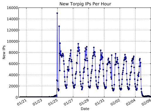
Figure 4: New unique IP addresses per hour
