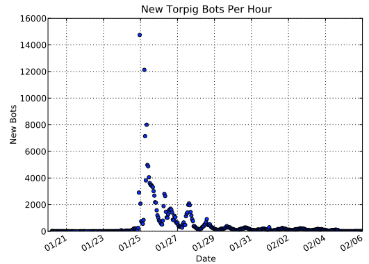
Figure 5: New bots per hour
