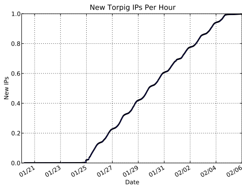
Figure 6: CDF New unique IP addresses per hour
