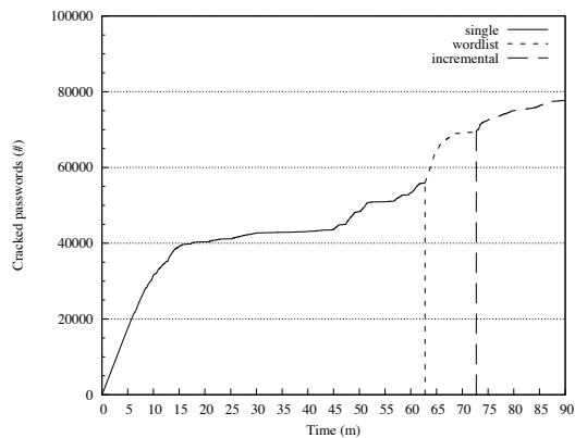
Figure 11: Number of passwords cracked in 90 minutes by the John the Ripper password cracker tool. Vertical lines indicate when John switches cracking mode. The first vertical line represents the switching from simple transformation techniques ("single" mode) to wordlist cracking, the second from wordlist to brute-force ("incremental").
