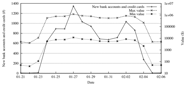
Figure 9: The arrival rate of financial data.
