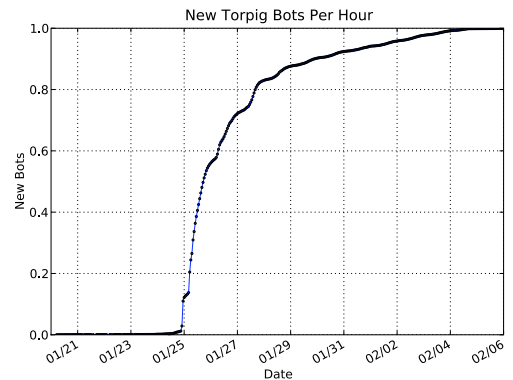
Figure 7: CDF New bots per hour
