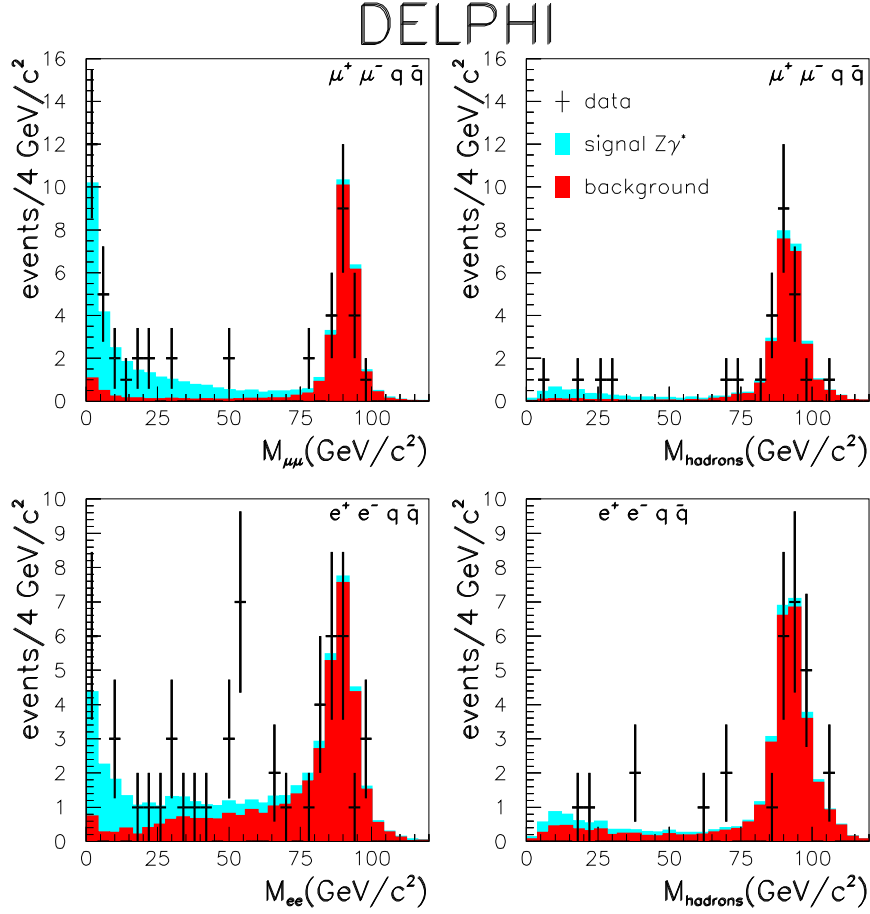
Figure 3: l^+l^-q\bar{q} final state: Distributions of the mass of one fermion pair when the mass of the second is within 15 GeV/c 2 of M_Z . The two lower plots are for the e^+e^-q\bar{q} channel and the two upper plots for the \mu^+\mu^-q\bar{q} channel. The points are the data summed over all energy points, the dark (red) histogram is the distribution of the background predicted by the Standard Model, and the light (light blue) histogram is the predicted distribution of the Z\gamma^* signal.
