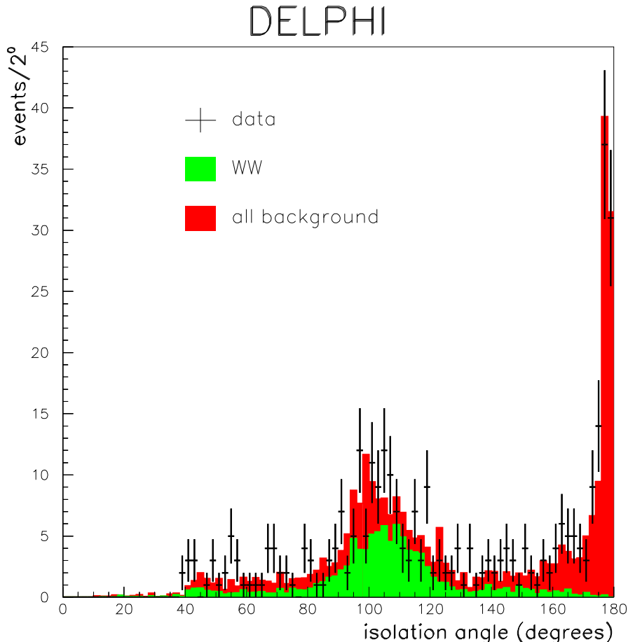
Figure 9: Isolation angle of selected electrons, muons and single charged-particle tracks in the sample selected to mimic the background to the selected q\bar{q}\nu\bar{\nu} sample. The points are the data, summed over all energy points, the light (green) histogram is the predicted WW contribution, and the dark (red) histogram is the rest of the background.
