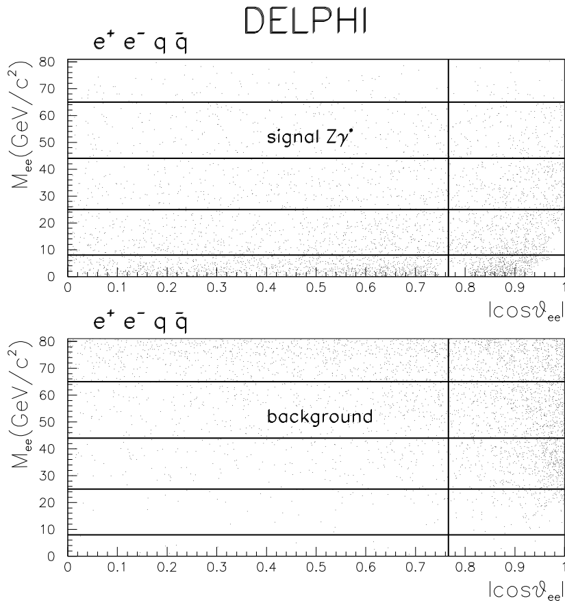
Figure 5: Distributions of the mass of the electron-positron pair in e^+e^-q\bar{q} events for values of M_{ee} less than 80 \text{ GeV}/c^2 versus the polar direction of the pair for signal Z\gamma^* (upper plot) and background (lower plot) when the mass of the hadronic system is compatible with the Z mass. The plot shows the predictions of the Standard Model, averaged over all energy points. The binning adopted for these events follows that in figure 4 with an additional division into barrel and endcap regions, described in detail in the text.
