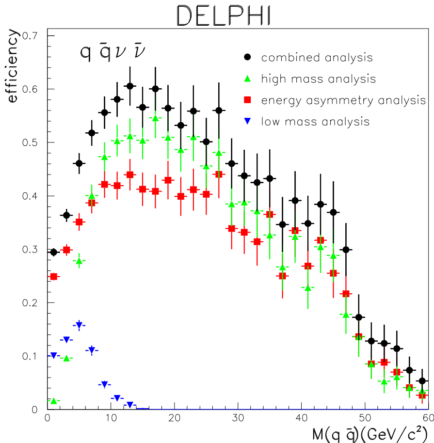
Figure 7: Selection efficiency of the q\bar{q}\nu\bar{\nu} analyses, averaged over all energy points, as a function of the generated M(q\bar{q}) mass. The efficiency is shown for each of the three analyses (see text) separately, and for the combined analysis.
