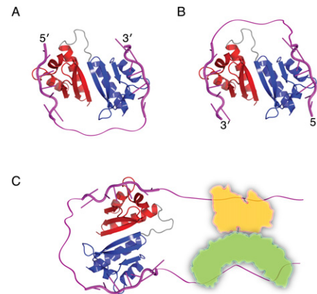
Figure 7. Model for RNA looping induced by binding of the ZBP1 KH34 domain and the assembly of RNA-protein complexes. (A,B) Current data allows two distinct modes of RNA binding to be modeled based on which sequences within the bipartite RNA element the individual KH domains interact with. Polarity of the RNA to the KH domains is conserved in both models. (C) Looping of the transcript may form the binding sites for additional RNA-binding proteins and nucleate the assembly of larger RNPs.
