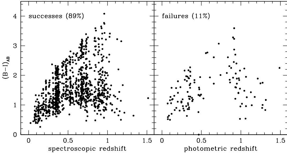
FIG. 8.—Distribution in color-redshift space of the objects for which a redshift was successfully obtained ( left ) and those for which a redshift was not obtained ( right ), plotting the latter at their photometric redshift. Objects in Classes 2 and 1 with a consistent photometric redshift defined to be |z_s - z_p| < 0.1(1 + z) as in Fig. 7 are counted as successes and those with an inconsistent photometric redshift, plus the Class 0 objects, are counted as failures.
