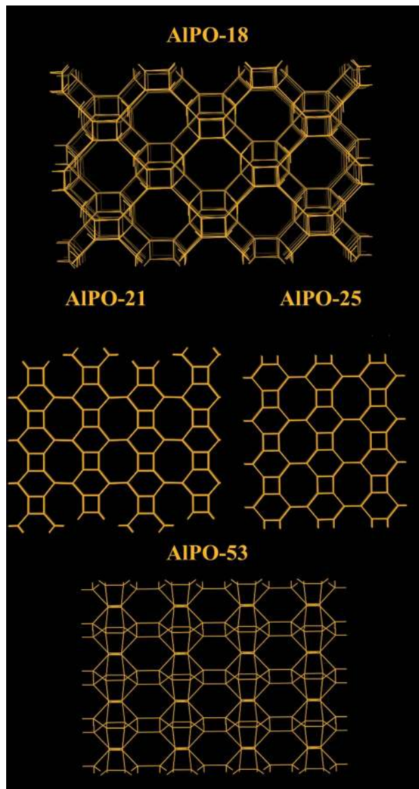
Fig. 12 Structure representation of AIPO-18 (AEI), AIPO-21 (AWO), AIPO-25 (ATV) and AIPO-53 (AEN), the yellow lines represent covalent bonds between two metal (Al or P) atoms (bridging O atoms), oxygen atoms are purposely omitted in order to show the pore system more clearly. Note that AIPO-21 transforms to AIPO-25 upon calcination.
