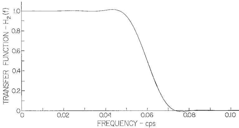
FIG. 3. Transfer function H_2(f) for Ormsby filter ( f_C = 0.05 cps, f_T = 0.07 cps) with 250 weights over the filtering interval T_w = 100 sec.
