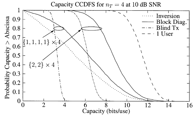
Fig. 3. Complementary cumulative distribution functions of sum capacity for Gaussian channels for four transmitters.
