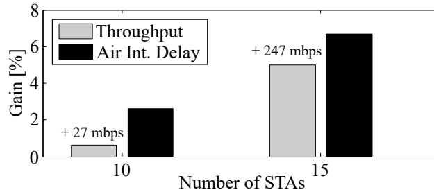
Figure 5.7: UDP Downlink Results
