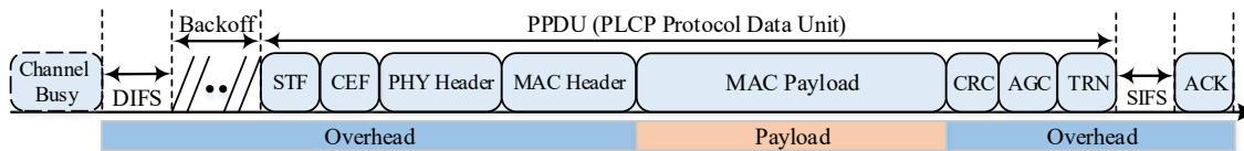
Figure 2.1: IEEE 802.11ad frame structure.
