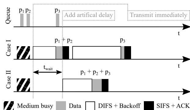
Figure 5.1: Aggregation Opportunity Example.
