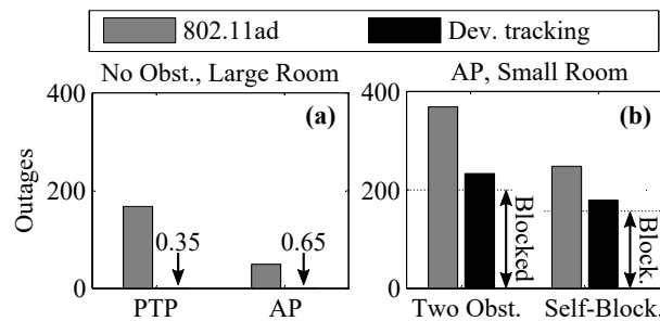
Figure A.4: Number of outages due to steering misalignment and/or blockage. The arrows in (a) show the values of the bars that are too small to be legible. The arrows in (b) indicate the fraction of outage which occurs because of no working (reflected) path being available due to the blockage.
