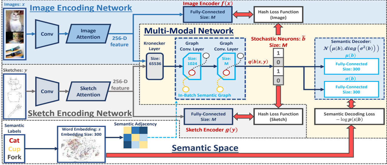
Figure 2. The deep network structure of ZSIH. The image (in light blue) and sketch encoding network (in grey) act as hash function for the respective modality with attention models [59]. The multi-modal network (in canary yellow) only functions during training. Sketch-image representations are fused by a Kronecker layer [22]. Graph convolution [30] and generative hashing techniques are leveraged to explore the semantic space for zero-shot SIBR hashing. Network configurations are also provided here.
