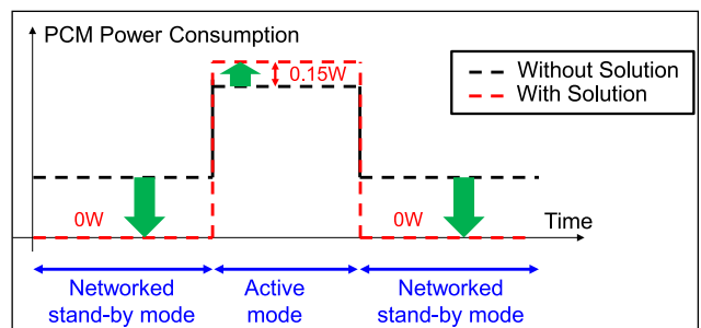
Fig. 15 Power consumption impact of PCM.
