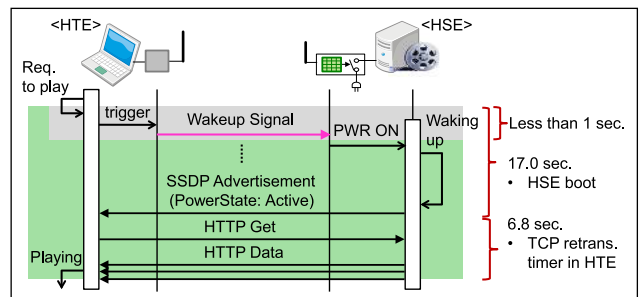
Fig. 14 Wake-up delay evaluation.
