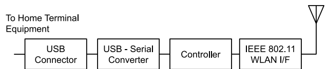
Fig. 8 WTM structure.
