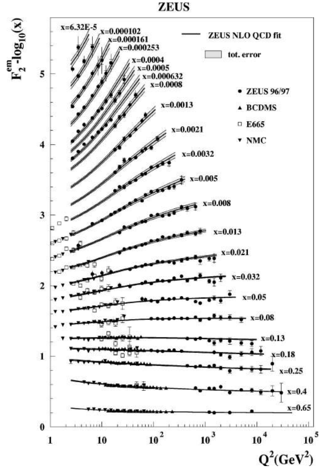
FIG. 2. The ZEUS-S NLO QCD fit compared to ZEUS96/97 and proton fixed-target F_2 data. The error bands are defined in the caption to Fig. 1.
