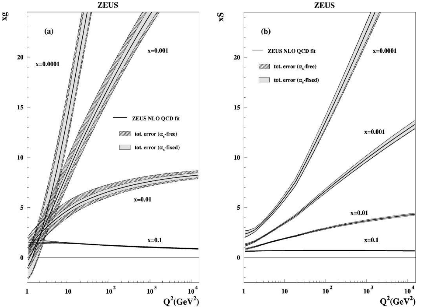
FIG. 11. (a) The gluon distribution from the ZEUS-S NLO QCD fit as a function of Q^2 for fixed x values. (b) The sea distribution from the ZEUS-S NLO QCD fit as a function of Q^2 for fixed x values. The error bands are defined in the caption to Fig. 6.
