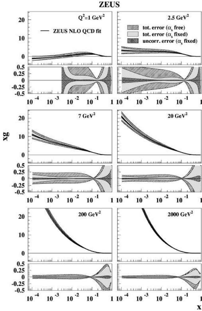
FIG. 9. The gluon distribution from the ZEUS-S NLO QCD fit for various Q^2 values. The error bands are defined in the caption to Fig. 6. The uncertainties on these distributions are shown beneath each distribution as fractional differences from the central value. Note that this uncertainty is not shown when the central value of the gluon distribution becomes negative.
