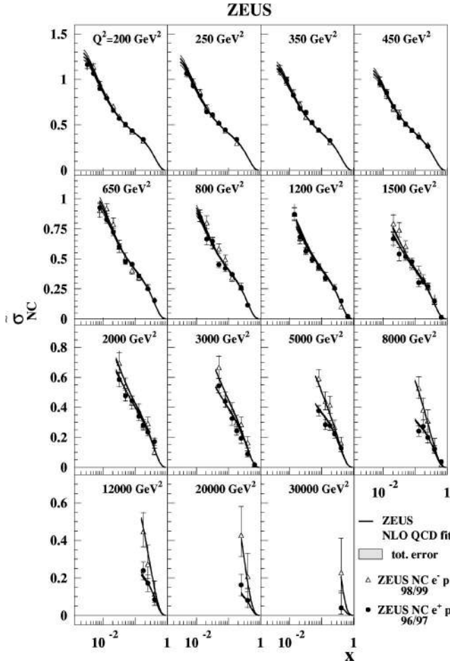
FIG. 3. The ZEUS-S NLO QCD fit compared to the ZEUS high- Q^2 e^+p and e^-p neutral current reduced cross sections. The error bands are defined in the caption to Fig. 1. Note that the e^+p data were taken at \sqrt{s}=300 GeV, whereas the e^-p data were taken at \sqrt{s}=318 GeV.
