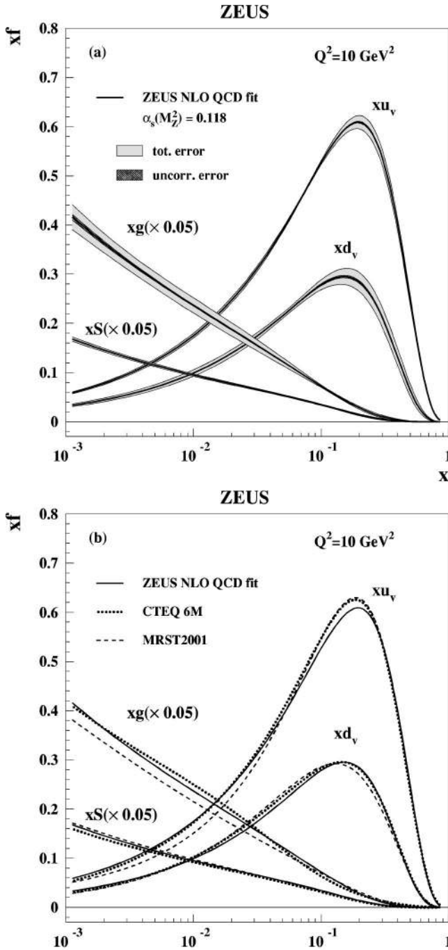
FIG. 5. (a) The gluon, sea, and u and d valence distributions extracted from the standard ZEUS-S NLO QCD fit at Q^2 = 10 \text{ GeV}^2 . The error bands in this figure show the uncertainty from statistical and other uncorrelated sources separately from the total uncertainty including correlated systematic uncertainties. (b) The gluon, sea, and u and d valence distributions extracted from the ZEUS-S NLO QCD fit at Q^2 = 10 \text{ GeV}^2 , compared to those extracted from the fits MRST2001 [5] and CTEQ6 [6].
