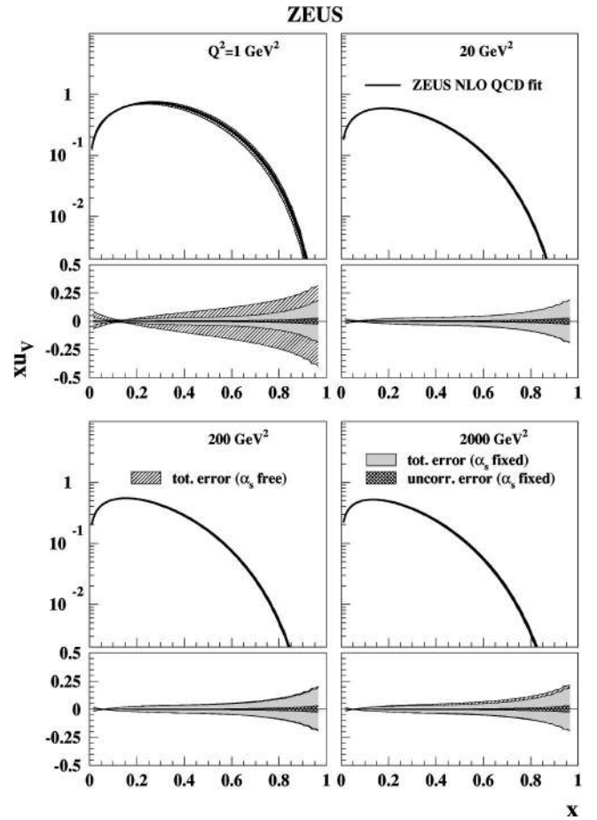
FIG. 6. The xu_v distribution from the ZEUS-S NLO QCD fit. The cross-hatched error bands show the statistical and uncorrelated systematic uncertainty, the gray error bands show the total experimental uncertainty including correlated systematic uncertainties (both evaluated from the ZEUS-S fit), and the hatched error bands show the additional uncertainty coming from variation of the strong coupling constant \alpha_s(M_Z) (evaluated from the ZEUS- \alpha_s fit). The uncertainties on these distributions are shown beneath each distribution as fractional differences from the central value.
