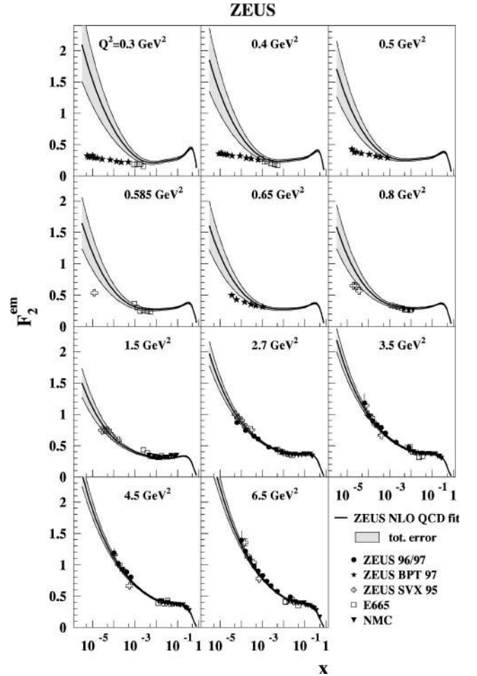
FIG. 15. F_2 data at very low Q^2 (including SVX95 and BPT97 data) compared to the backward extrapolated ZEUS-S NLO QCD fit. The error bands are defined in the caption to Fig. 1.
