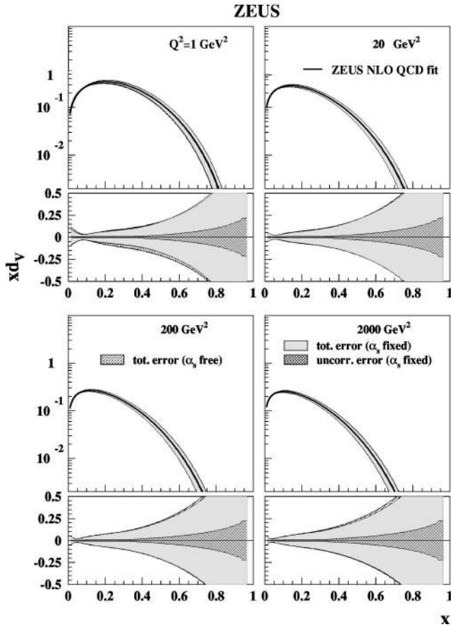
FIG. 7. The x d_v distribution from the ZEUS-S NLO QCD fit. The error bands are defined in the caption to Fig. 6]. The uncertainties on these distributions are shown beneath each distribution as fractional differences from the central value.
