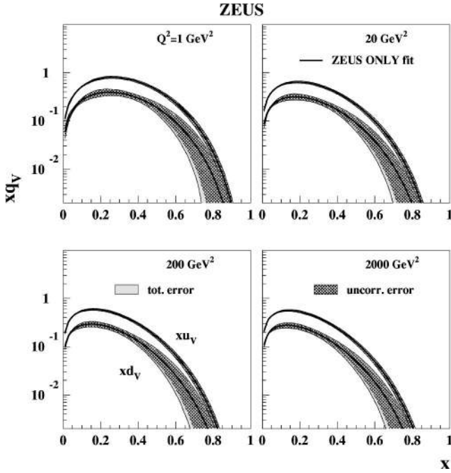
FIG. 14. The xu_v and xd_v distributions from the ZEUS-S NLO QCD fit. The error bands are defined in the caption to Fig. 13. The value of \alpha_s(M_Z) = 0.118 is fixed.
