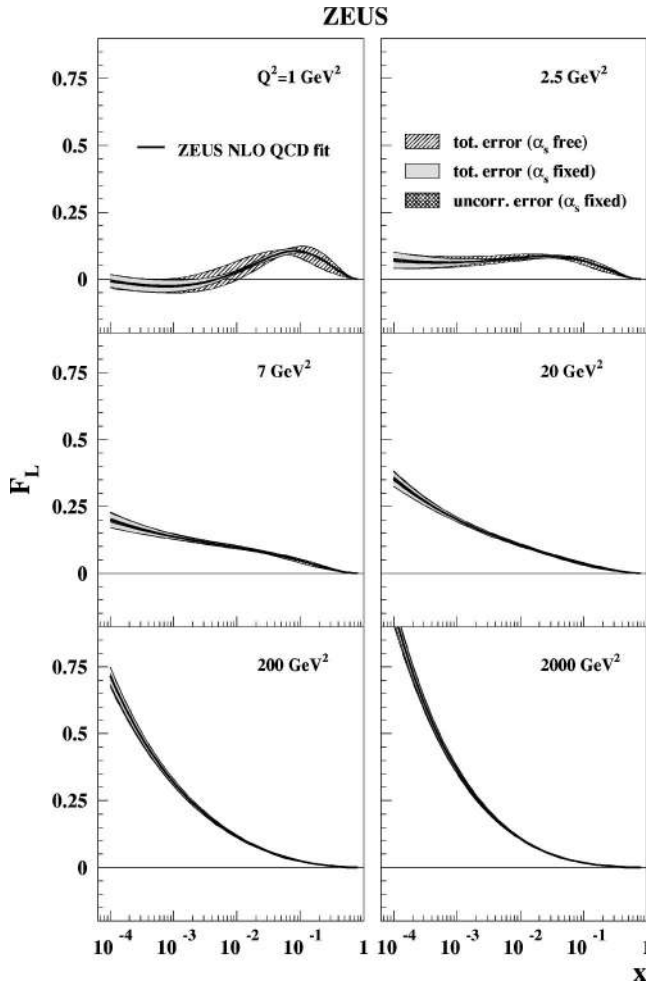
FIG. 12. The longitudinal structure function F_L from the ZEUS-S NLO QCD fit. The error bands are defined in the caption to Fig. 6.
