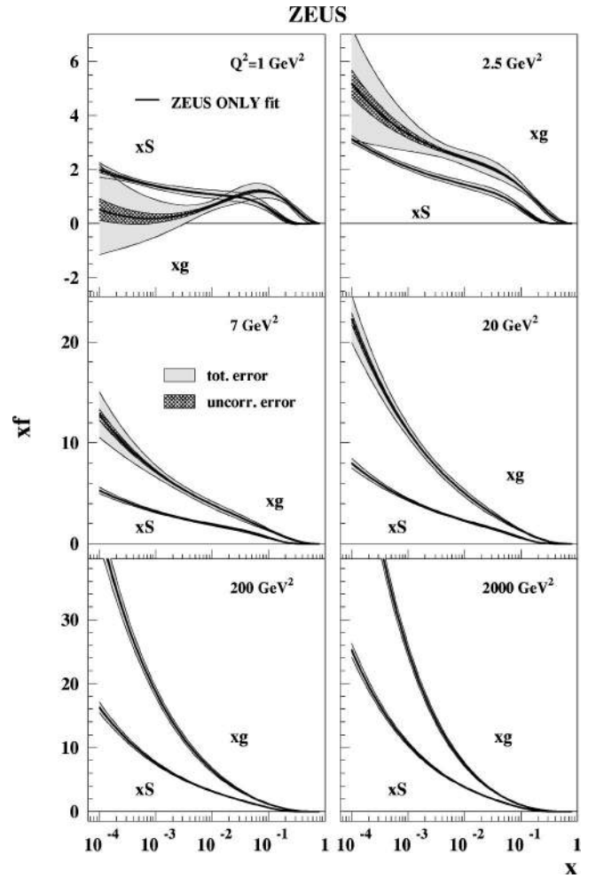
FIG. 13. The gluon and sea distributions from the ZEUS-S NLO QCD fit in various Q^2 bins. The error bands show the uncertainty from statistical and other uncorrelated sources separately from the total uncertainty including correlated systematic uncertainties. The value of \alpha_s(M_Z) = 0.118 is fixed.
