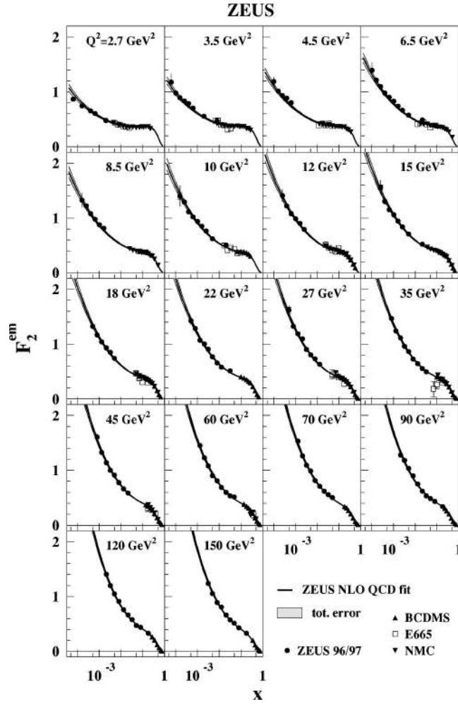
FIG. 1. The ZEUS-S NLO QCD fit compared to ZEUS 96/97 and proton fixed-target F_2 data. The error bands of the fit represent the total experimental uncertainty from both correlated and uncorrelated sources.
