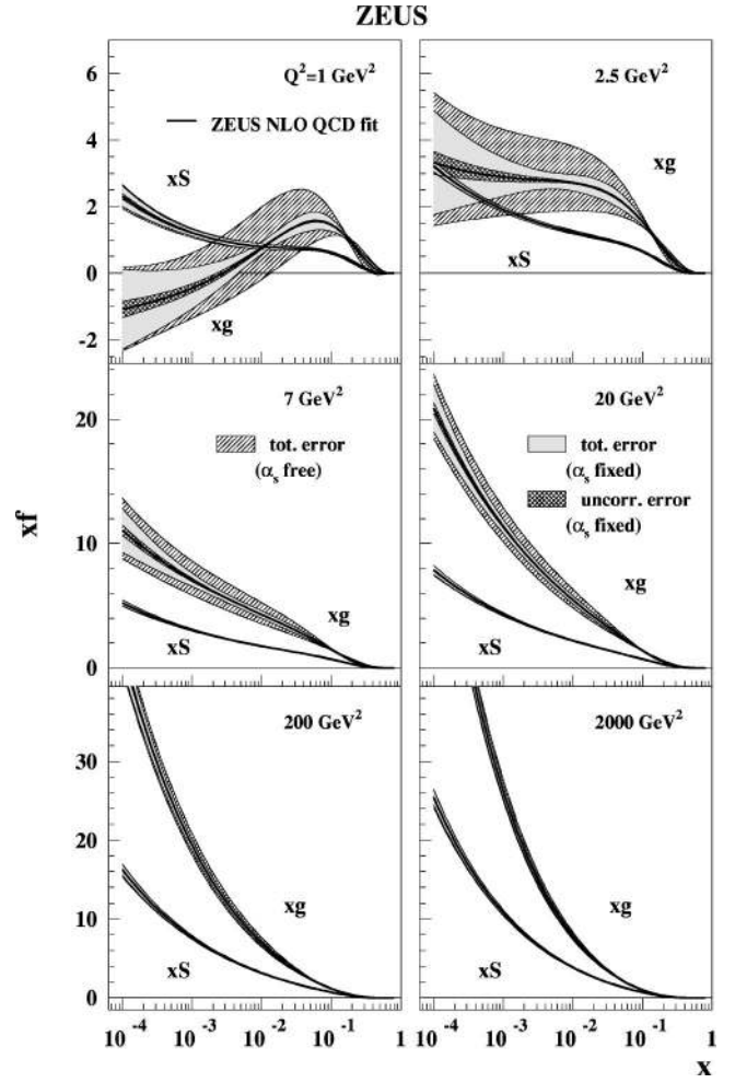
FIG. 10. Comparison of the gluon and sea distributions from the ZEUS-S NLO QCD fit for various Q^2 values. The error bands are defined in the caption to Fig. 6.
