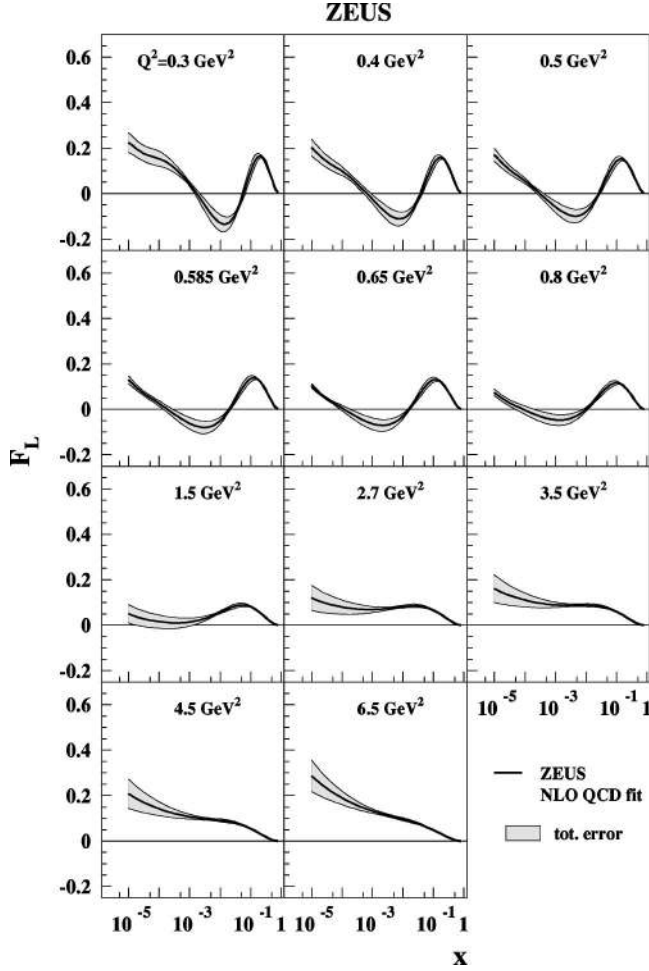
FIG. 16. The predictions for F_L at very low Q^2 from the backward extrapolated ZEUS-S NLO QCD fit. The error bands are defined in the caption to Fig. 1.
