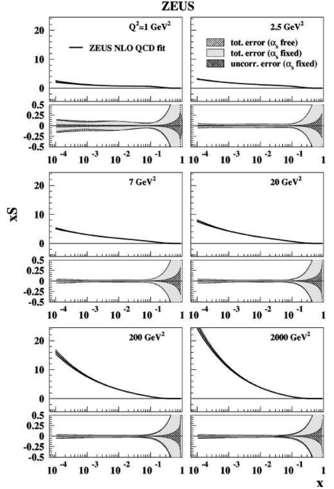
FIG. 8. The sea distribution from the ZEUS-S NLO QCD fit for various Q^2 values. The error bands are defined in the caption to Fig. 6. The uncertainties on these distributions are shown beneath each distribution as fractional differences from the central value.
