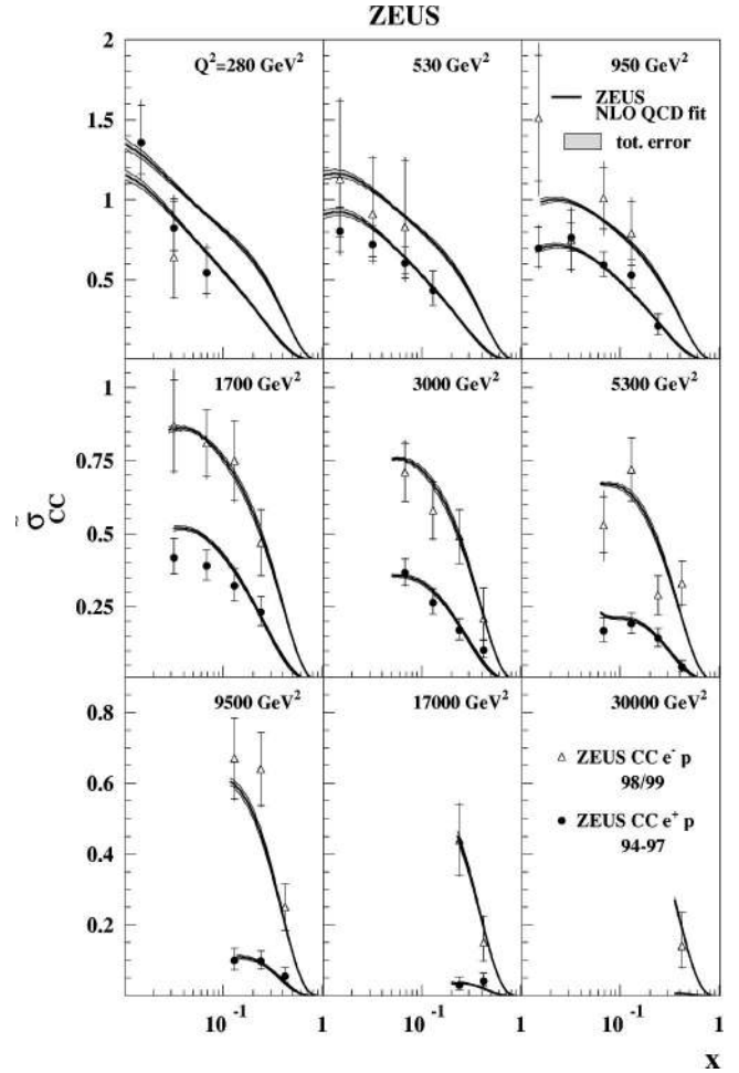
FIG. 4. The ZEUS-S NLO QCD fit compared to the ZEUS high- Q^2 e^+p and e^-p charged current reduced cross sections. The error bands are defined in the caption to Fig. 1. Note that the e^+p data were taken at \sqrt{s}=300 GeV, whereas the e^-p data were taken at \sqrt{s}=318 GeV.
