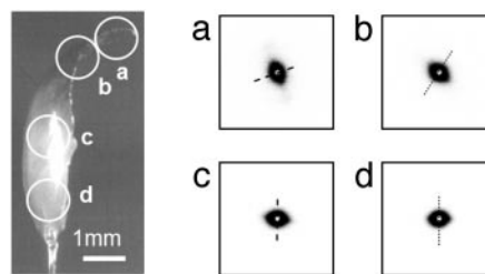
Fig. 3. SAXS on Nereis jaw. (Left) Light microscopy image of a jaw mounted in the SAXS apparatus. The white circles indicate the approximate positions and diameter of sampled areas. (Right a-d ) SAXS patterns obtained from each point circled in Left. The anisotropic signal is indicative of a fiber-like structure, where the longitudinal axis of the fibers is oriented along the short axis of the scattering pattern (dashed line). The fiber axis follows the outline of the jaw.
