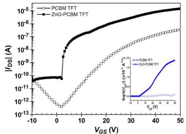
Fig. 11. Transfer I_{\text{DS}}-V_{\text{GS}} characteristics of pristine PCBM and ZnO-PCBM TFT devices in the saturation regime at V_{\text{DS}} = 40 V. The inset shows the I_{\text{DS}}^{1/2}-V_{\text{GS}} characteristics in the linear regime at V_{\text{DS}} = 10 V.
