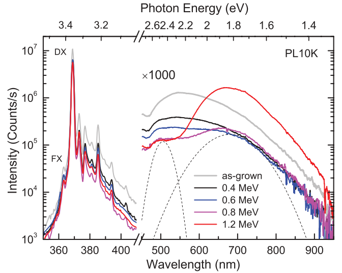
FIG. 2. (Color online) PL spectra from electron irradiated samples measured at 10 K. Note a \times 1000 prefactor for the deep level related emission components. Dashed lines indicate the position and width of the observed red and green emission bands. FX and DX denote free and donor-bound exciton recombination, respectively.
