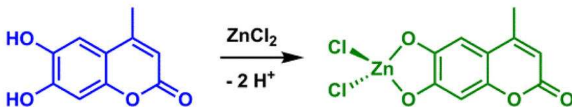
Scheme 3. Methylsculetin undergoes deprotonation upon forming a Zn(II) complex. 121
