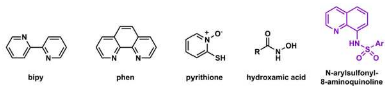
Fig. 25. A few bidentate ligands for Zn(II).
