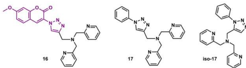
Fig. 20. 1,2,3-Triazolyl-containing tetridentate 16 and 17 , and tridentate iso-17 . 191
