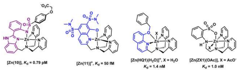
Fig. 15. Zn(II) complexes of a few pentadentate ligands 10 , 138 11 , 162 HQ1 , 167 and ZX1 , 168 with K_d values shown.
