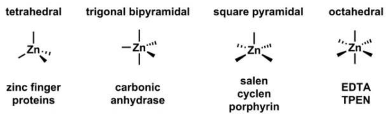
Fig. 12. Zn(II) coordination geometry in various ligand environments.
