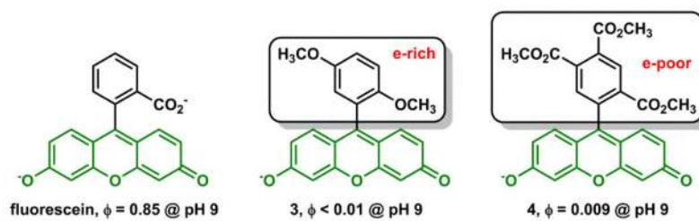
Fig. 6. The phenyl component determines the fluorescence quantum yield of the xanthen moiety. 87,88
