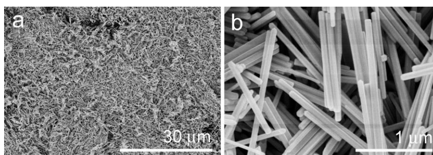
Fig. S3 (a) and (b) SEM image showing the ZnO nanorod.
