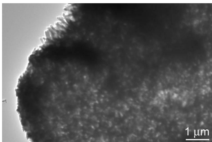
Fig. S2 TEM images show that the ZnO nanorod arrays are assembled on the graphene sheets' surfaces.
