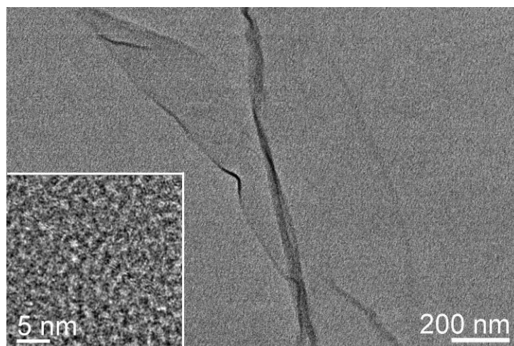
Fig. S1 TEM image shows a rGs; the inset shows that the rGs is multi-layered.
