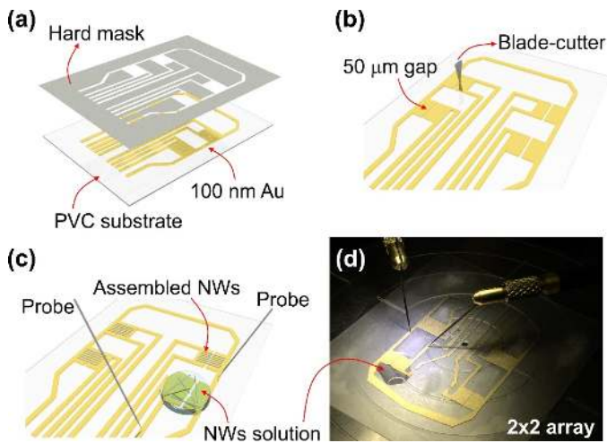
Fig. 2. (a-c) 3D schema of PD fabrication steps: (a) electrodes patterning by hard-masking; (b) electrodes gap patterning by blade-cutting; (c) NWs solution drop-casting and DEP assembly of ZnO NWs. (d) Image of ZnO NWs assembled by DEP between Au electrodes, forming a 2 \times 2 array of UV PDs.
