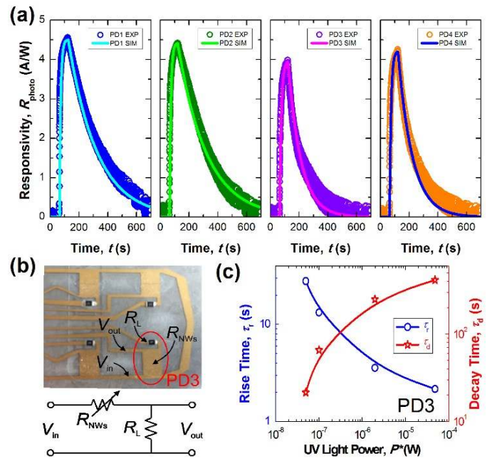
Fig. 5. (a) R_{\text{photo}} vs. time for PD1-4, using a V_{\text{in}} = 5\text{ V} , R_L = 100\ \text{M}\Omega , and a P^* = 1\ \mu\text{W} . (b) Image of 2 \times 2 UV PDs array (top) and equivalent circuit diagram (bottom). (c) \tau_r and \tau_d vs. P^* for PD3.
