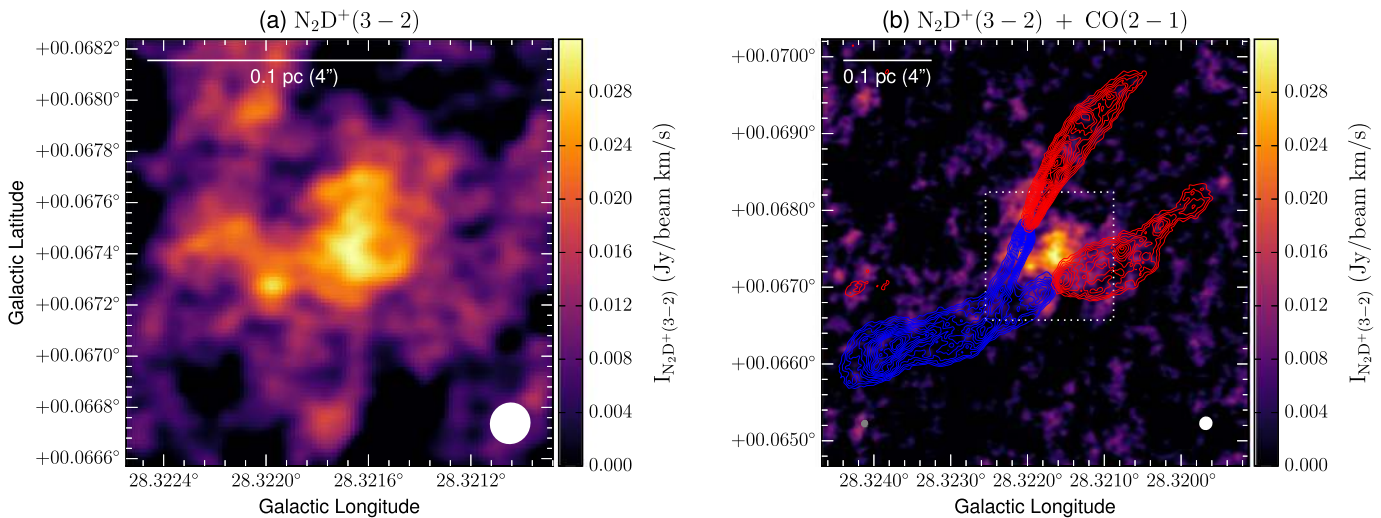
Figure 15. (a) Zoom-in view of Figure 3(c). The synthesized beam ( \sim 0.4'' ) is shown as a white filled ellipse at lower right. (b) CO(2–1) zeroth-moment contours overlaid on Figure 3(c). The contour map is the same as Figure 12(b), except for starting from 15\sigma . The synthesized beam is shown in the lower right corner as a white filled ellipse. The dotted square shows the zoom-in region of panel (a).
