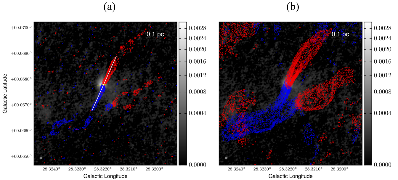
Figure 12. CO(2–1) zeroth-moment contours overlaid on the continuum images (grayscale with units of \text{Jy beam}^{-1} , showing combined data from Figure 1), showing combined data from Figure 1). Blue contours show emission integrated from 33.8 to 72.8 \text{ km s}^{-1} ; red contours show emission integrated from 85.8 to 124.8 \text{ km s}^{-1} . The displayed contour levels are 5\sigma , 7.5\sigma , 10\sigma , 12.5\sigma .... (a) Outflow contours from extended-configuration-only data (maximum contour level 25\sigma with \sigma = 16 \text{ mJy beam}^{-1} \text{ km s}^{-1} ). (b) Outflow contours from combined data (maximum contour level 45\sigma with \sigma = 12 \text{ mJy beam}^{-1} \text{ km s}^{-1} ). The synthesized beams are shown in the lower left corners as gray filled ellipses.
