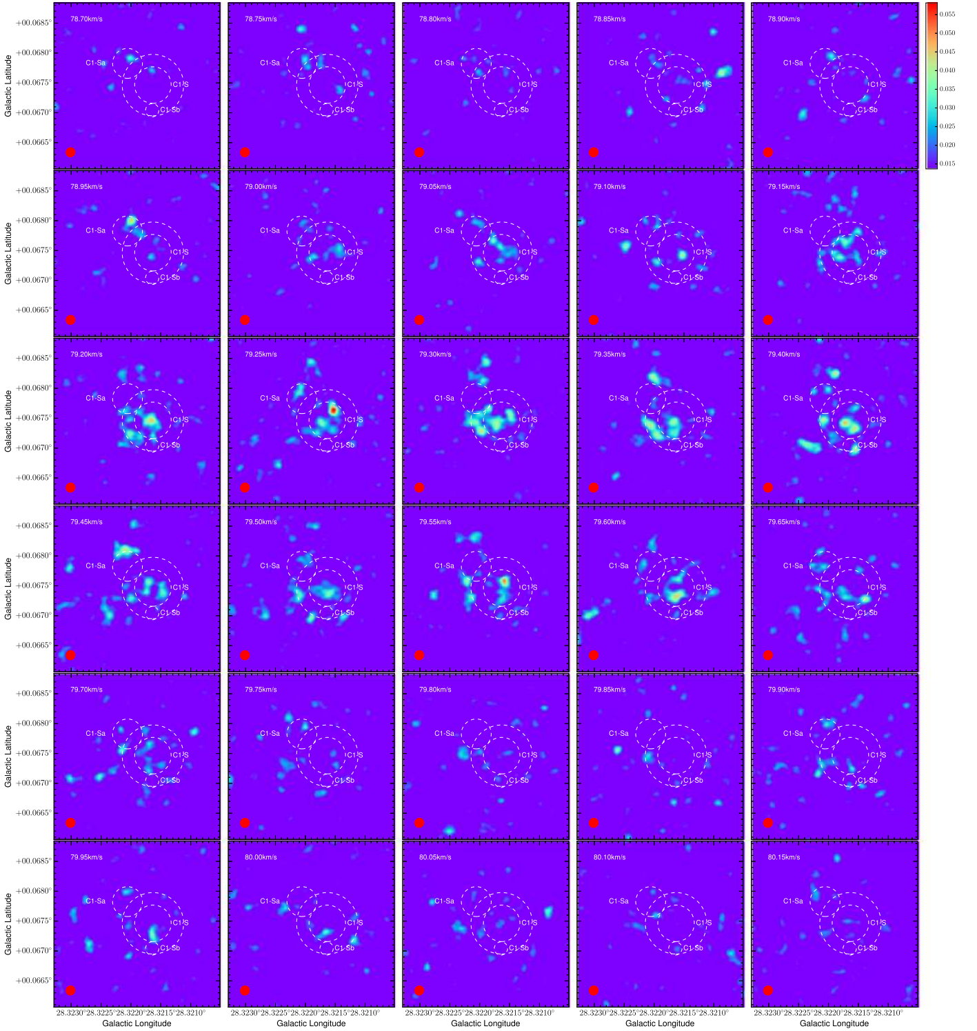
Figure 8. Same as Figure 7, but with the N_2D^+(3-2) data uv-tapered to \sim 0.5'' resolution. In this case, \sigma = 0.008 Jy beam ^{-1} .
