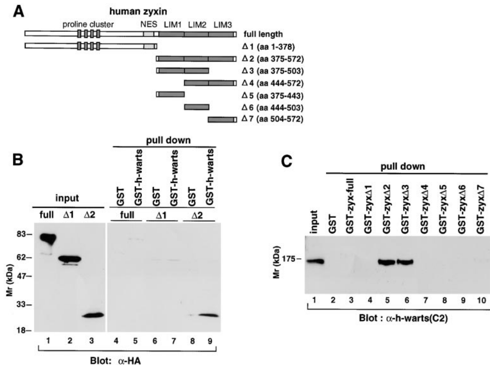
Figure 2. In vitro interaction of h-warts/LATS1 and zyxin. (A) Schematic diagram of deletion mutant zyxin showing their domain structures. The NH 2 -terminal two-thirds mutant (Δ1) contains four copies of a proline rich cluster and the nuclear exporting signal (NES), and the COOH-terminal third mutant (Δ2) contains three copies of the LIM domain. LIM domains were constructed tandemly or independently as indicated (Δ3–Δ7). The HA-tag epitope or the GST region of the fusion protein is not shown. (B) The lysates of COS7 cells expressing the indicated HA-tagged zyxin full-length and mutants (lanes 1–3) were subjected to incubation with either GST alone (lanes 4, 6, and 8) or GST-h-warts/LATS1 (amino acids 136–700) resin (lanes 5, 7, and 9). The bound fraction was analyzed by SDS-
